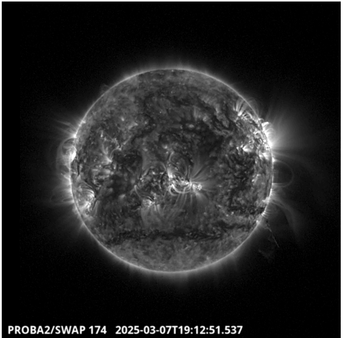
Filament eruption on the South_west limb of the solar disk around 19:13 UT. Find a movie of the events here (SWAP movie)
